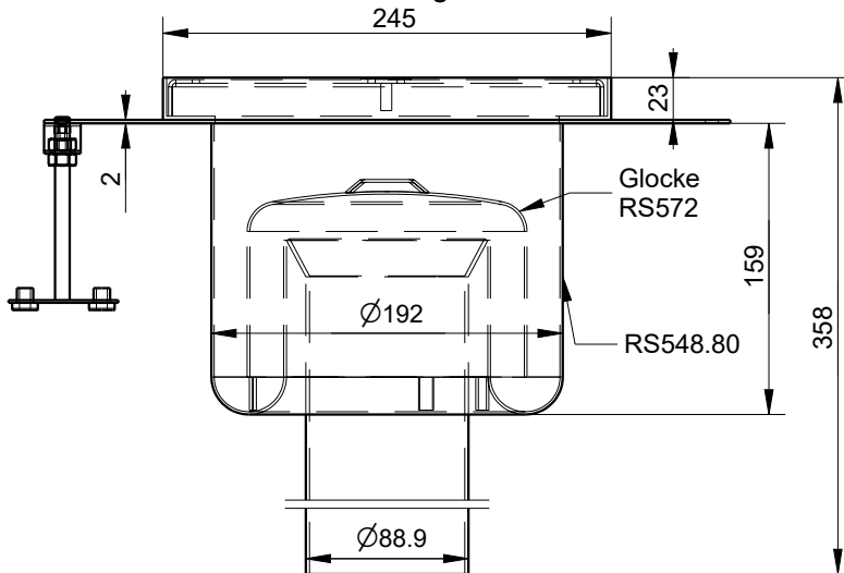
RS511.2.239
